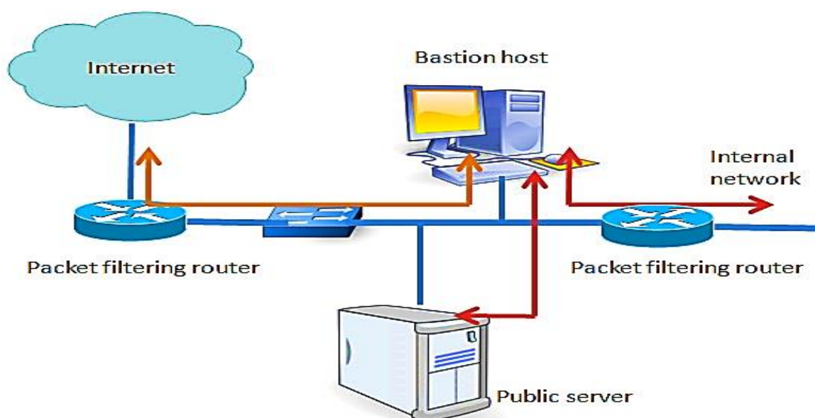
Fig. 5 Screened Host Firewalls
