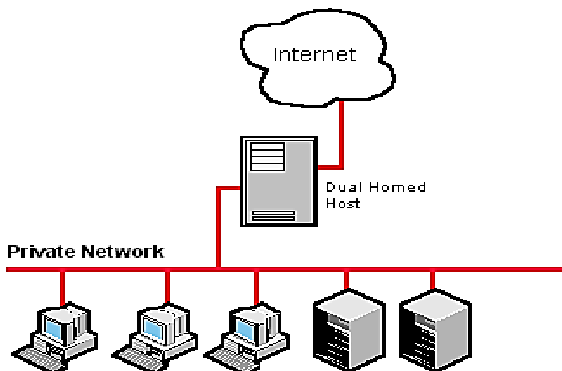
Fig.6 Dual-Homed Host Firewalls
