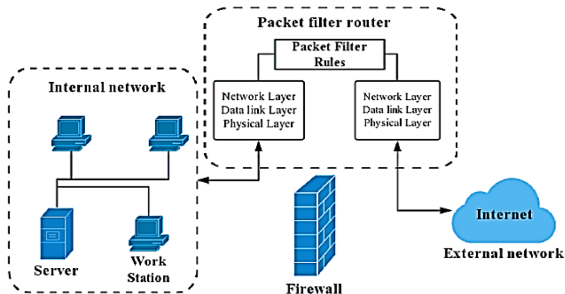
Fig. 4 Packet Filtering
