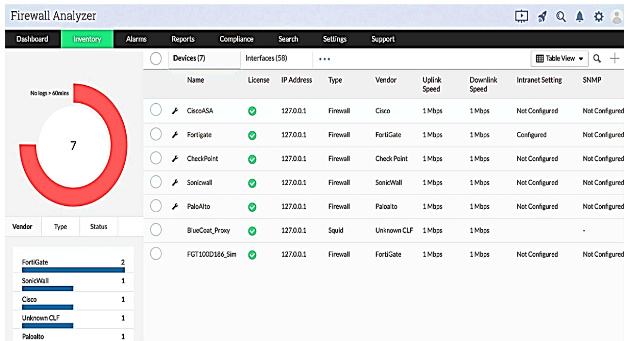
Fig. 8 Monitor Traffic
